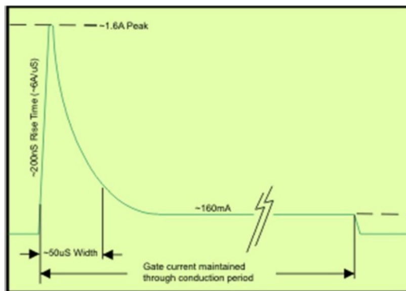
SCR Gate Drive Profile
