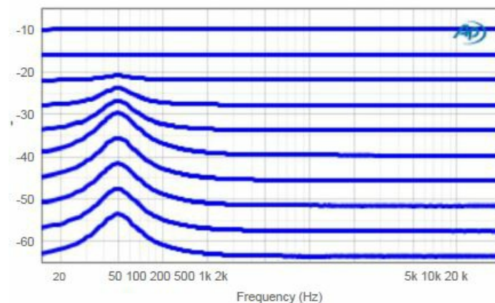
Frequency response correction of the loudness circuit
