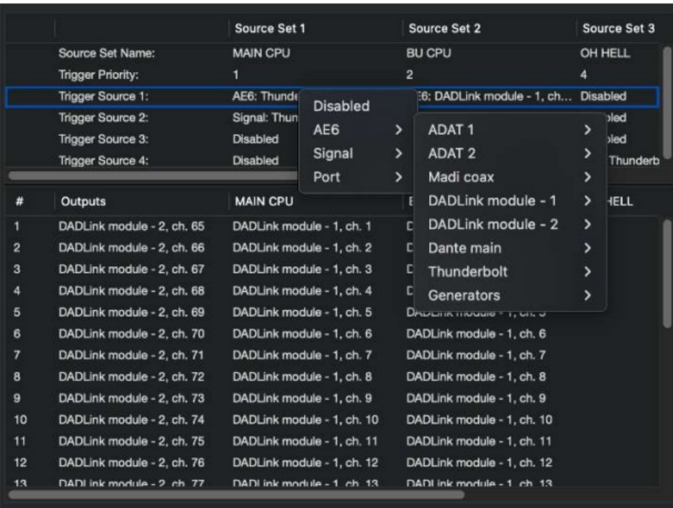
Figure 9, Trigger sources
