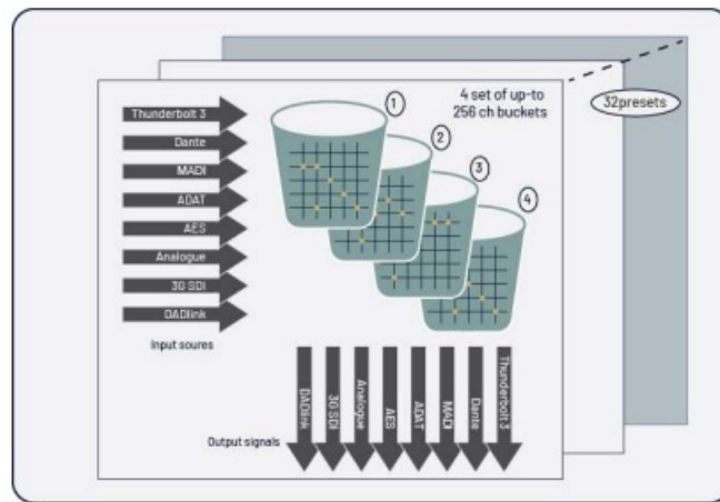
Figure 1, Routing presets and buckets
