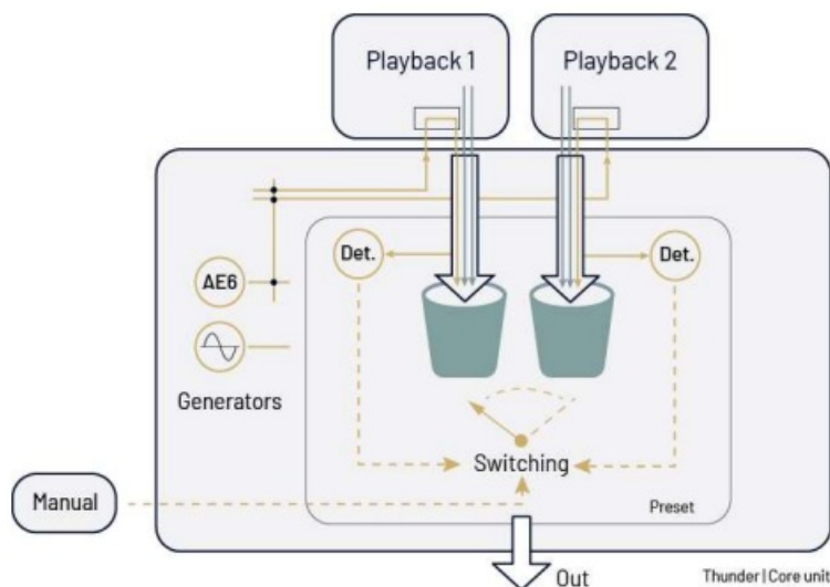
Figure 2, Detectors and automation example
