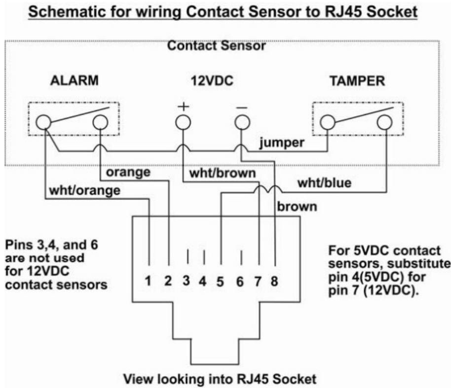
Figure 6- Contact sensor wired to RJ45 socket
