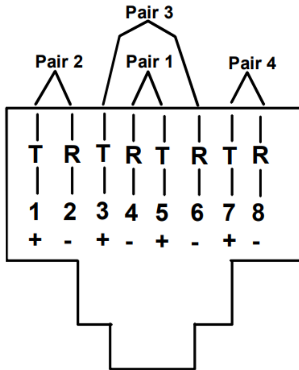
(View Looking into RJ45 Socket)
