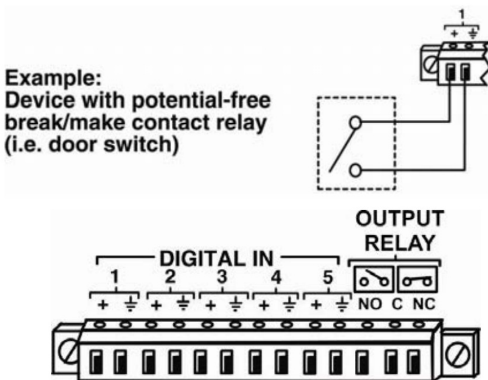
Figure 3- Terminal block for dry-contact sensors
