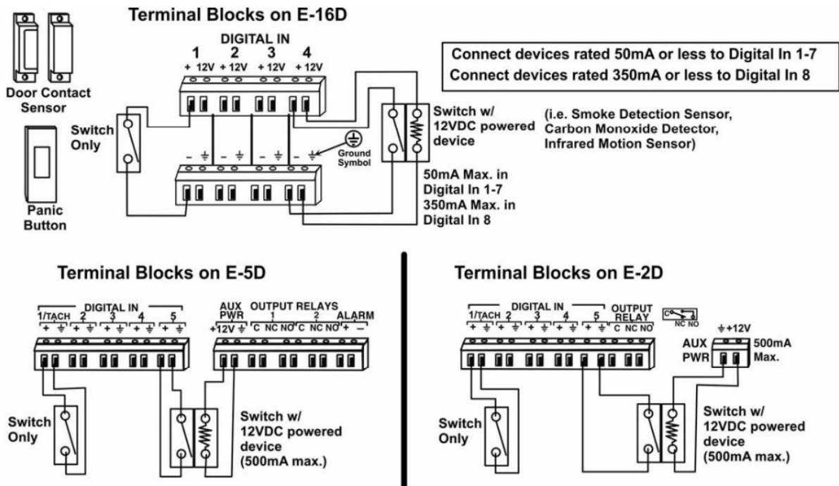
Figure 8- Basic DIGITAL IN Terminal Connections
