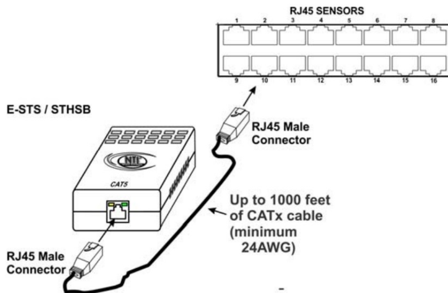
Figure 4- Sensors connected by cables with RJ45 connectors
