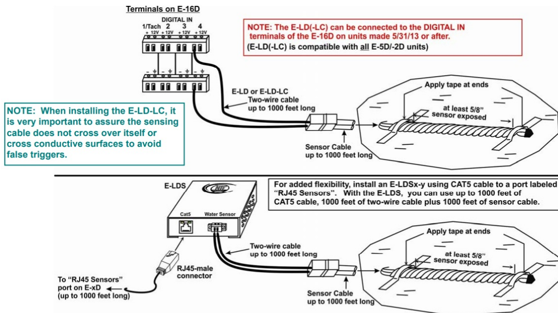
Figure 9- Secure liquid detection sensor with tape
