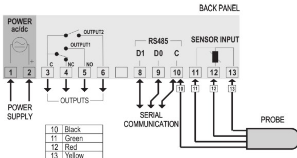
Fig. 2 – N322RHT terminals
