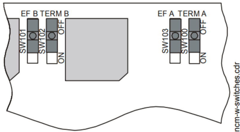
Figure 4 NCM-W Switches
