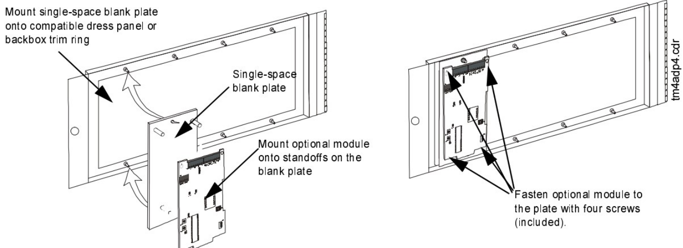
Mounting a Single-space Blank Plate onto the Dress Panel with Optional Module
