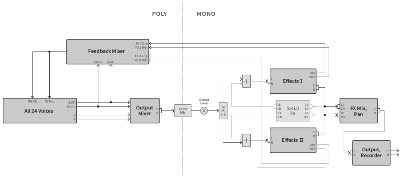
C15 Synth Engine – Layer/Split Sound Overview
