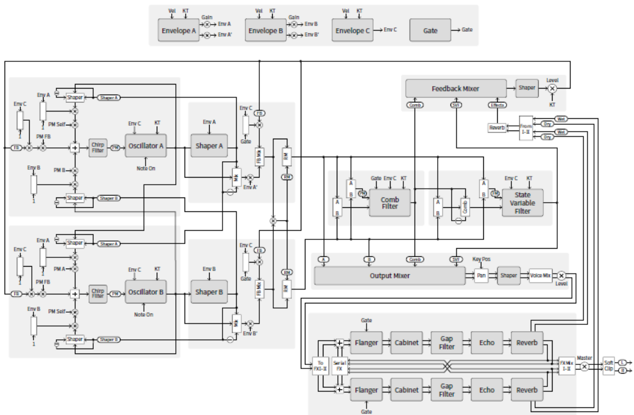
C15 Synth Engine – Single Sound Overview
