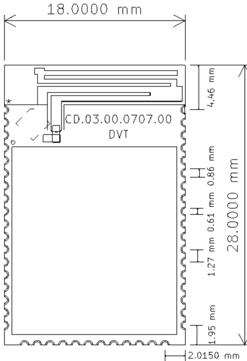
Figure 1.5 Dimensional specifications
