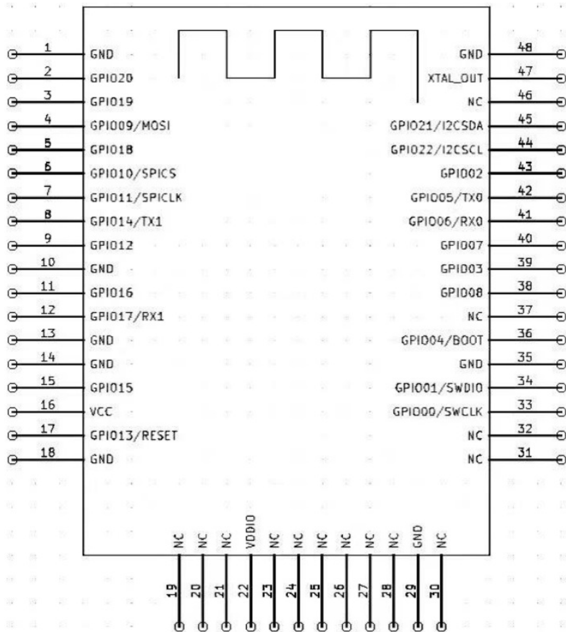
Figure 3.1 Pin Definition
