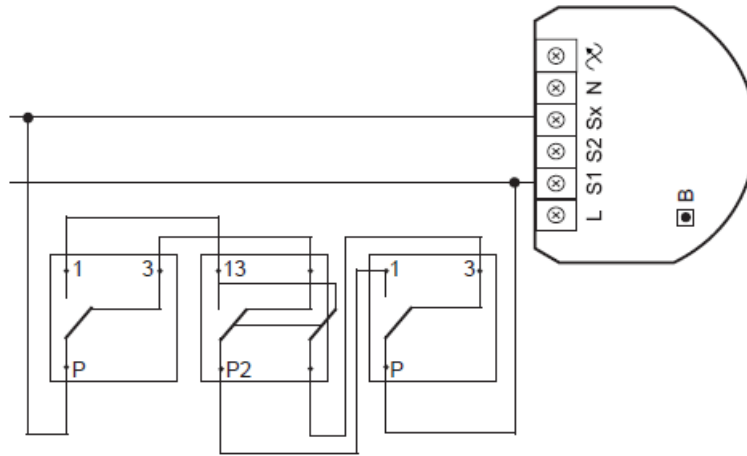
Fig. 4. Wiring diagram – 3-way switch connection
