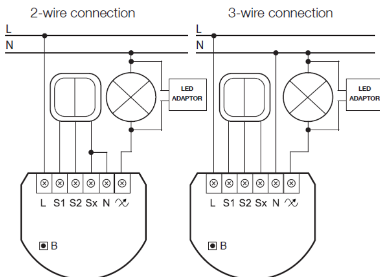
Fig. 3. Wiring diagram – connecting the LED Adaptor
