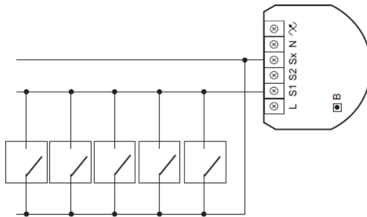
Fig. 5. Wiring diagram – momentary wall switches connection
