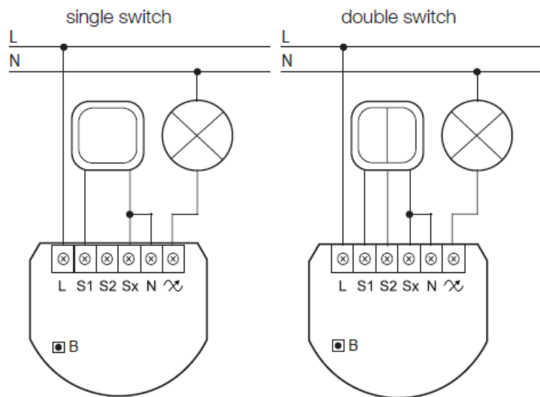
Fig. 1. Wiring diagram – 2-wire connection
