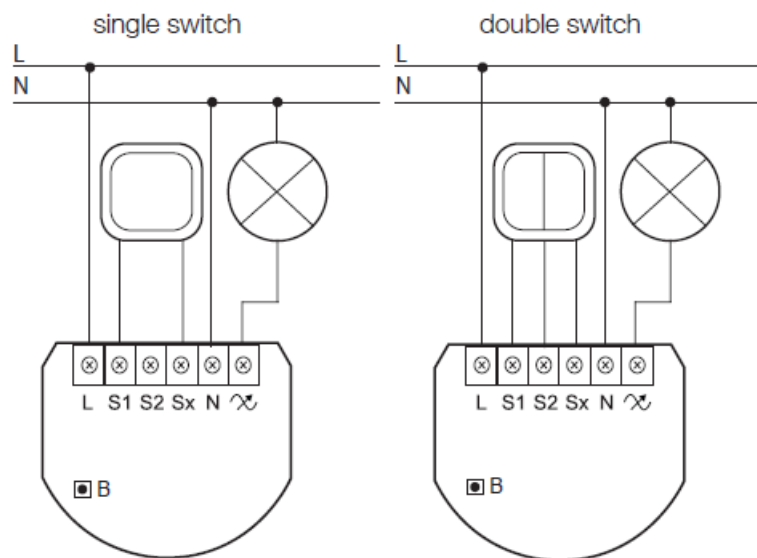
Fig. 2. Wiring diagram – 3-wire connection
