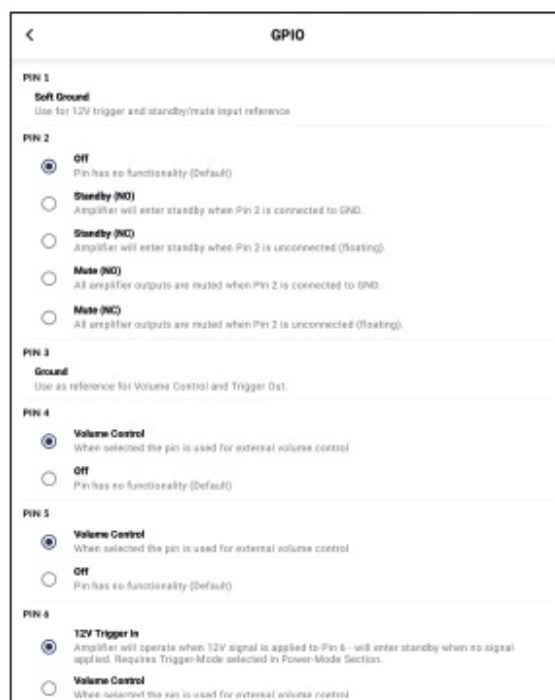
Diagram 5R Connections for remote standby/mute switch via GPIO.
