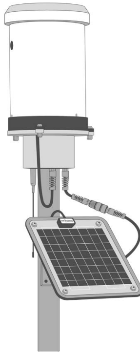
Connection of the G2-RTU external power cable and an SP-Series solar panel.
