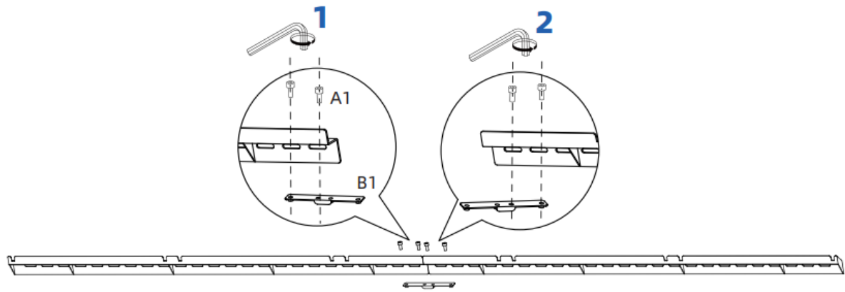
lower wall-mounting bracket
