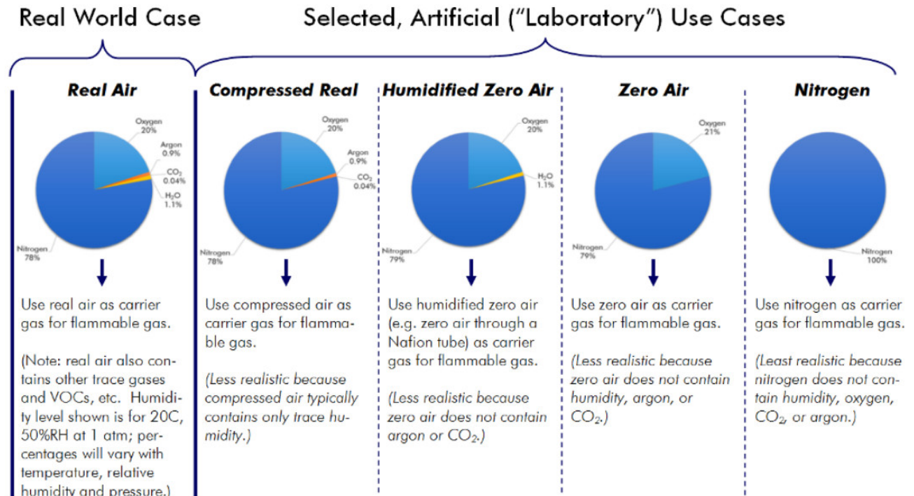
Figure 6: Various “air” options for use as the carrier, or background, gas during methane gas testing. The best practice is to use one of the options toward the left side of the figure. In addition, do not switch between two different types of “air” during an experiment, as this can produce unwanted (and unrealistic) testing artifacts.
