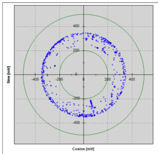
Excessive jitter/noise
