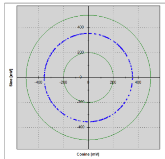
Low jitter/noise
