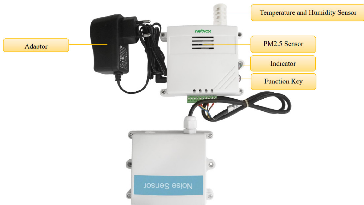
Fig. 1. RA0723 internal PM2.5 and temperature and humidity sensor, external noise Sensor (subject to the actual object)
