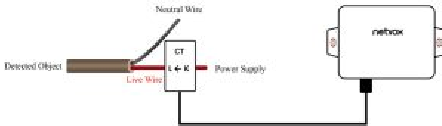
CT Wiring Schematic Diagram (Current direction K→L)
