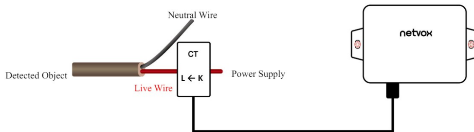
CT Wiring Schematic Diagram (Current direction K→L)
