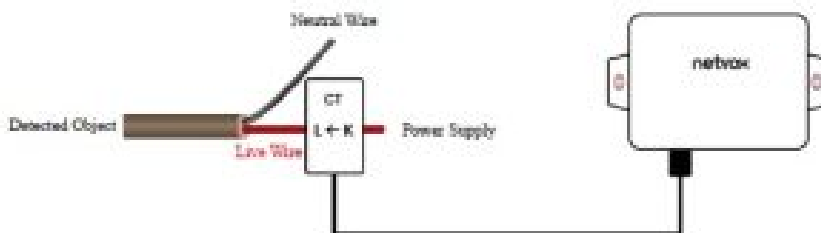
CT Wiring Schematic Diagram (Current direction K→L)
