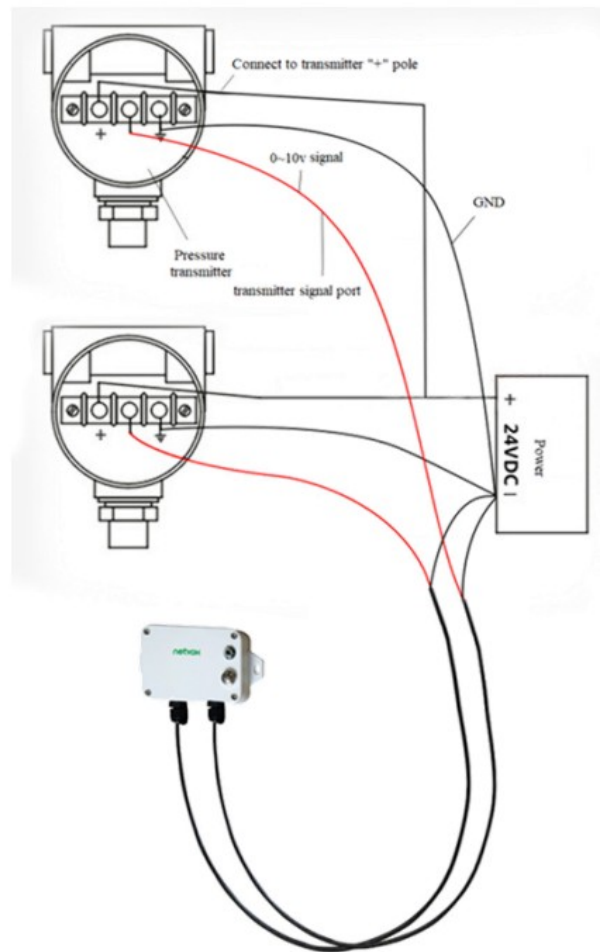
3-wire System Example Diagram
