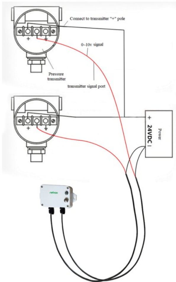
2-wire System Example Diagram
