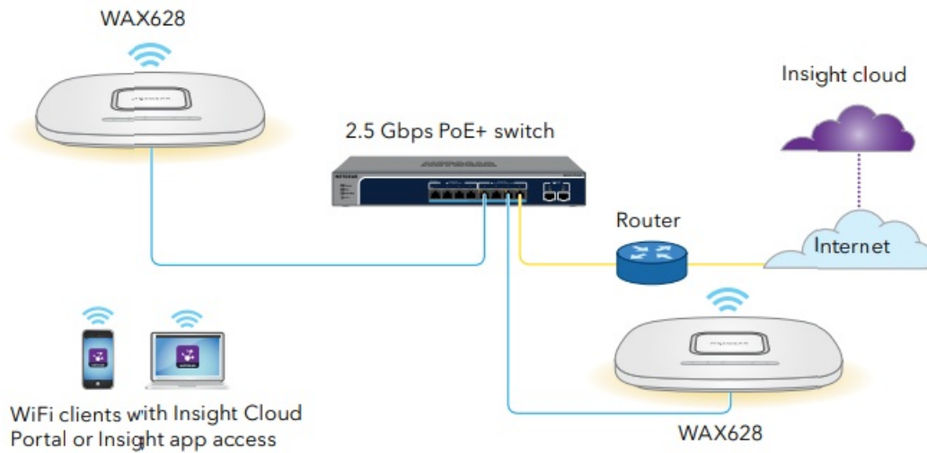
Sample connections for a standalone setup
