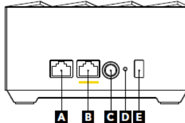
Router
