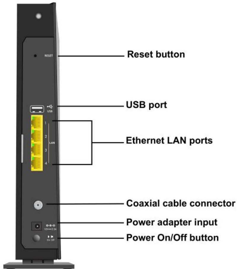
Figure 3. Modem router rear panel
