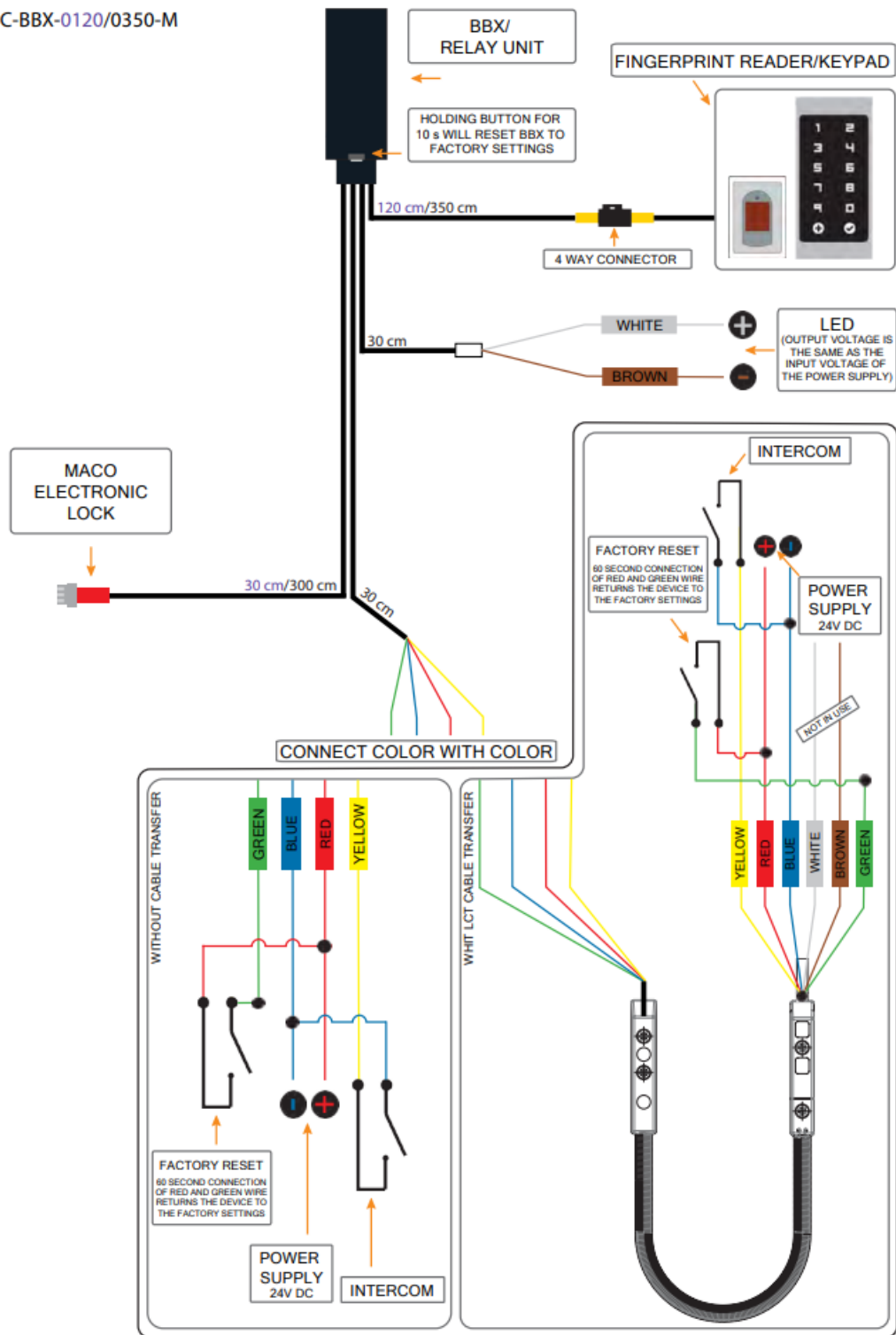
CONNECTION DIAGRAM: PRODUCTS IN COMBINATION WITH BBX MINI CONTROL UNIT (ROTO SH)
