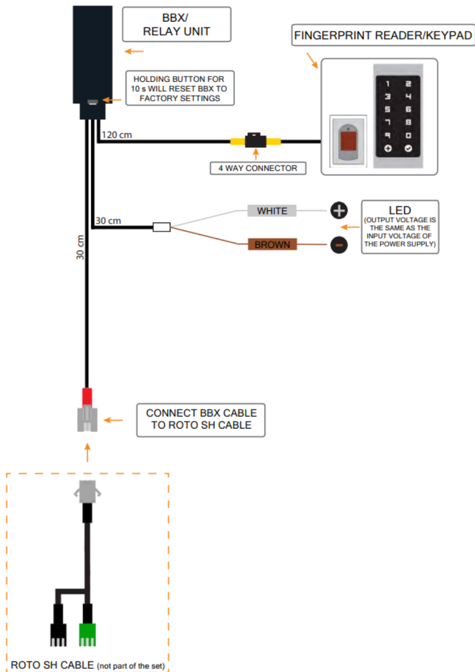
CONNECTION DIAGRAM: PRODUCTS IN COMBINATION WITH BBX MINI CONTROL UNIT (ROTO)
