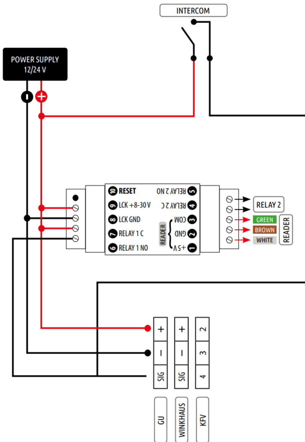
CONNECTION DIAGRAM: PRODUCTS – DIN CONTROL UNIT AND A MOTOR LOCK (MACO, FUHR)
