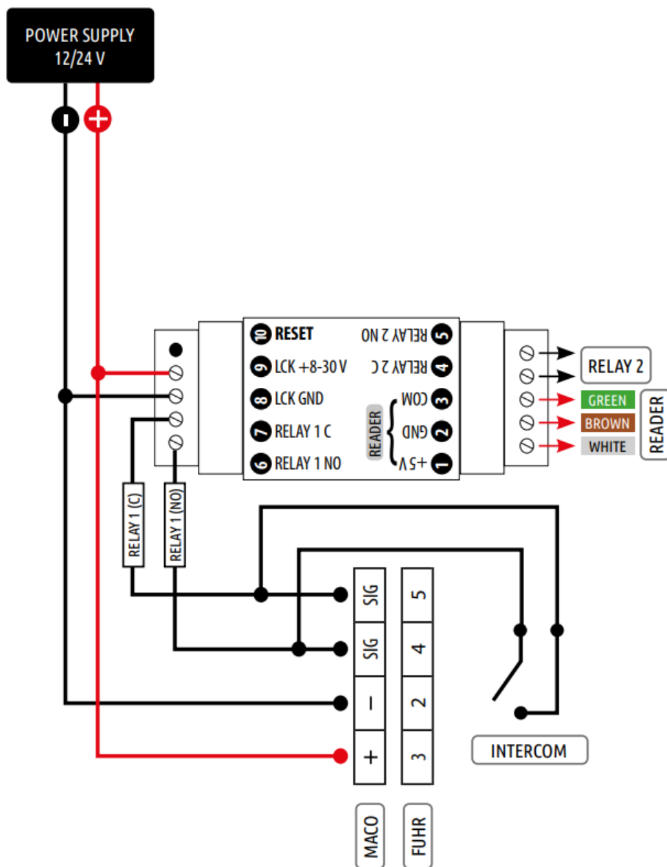
CONNECTION DIAGRAM: PRODUCTS – DIN CONTROL UNIT AND ELECTRIC STRIKE
