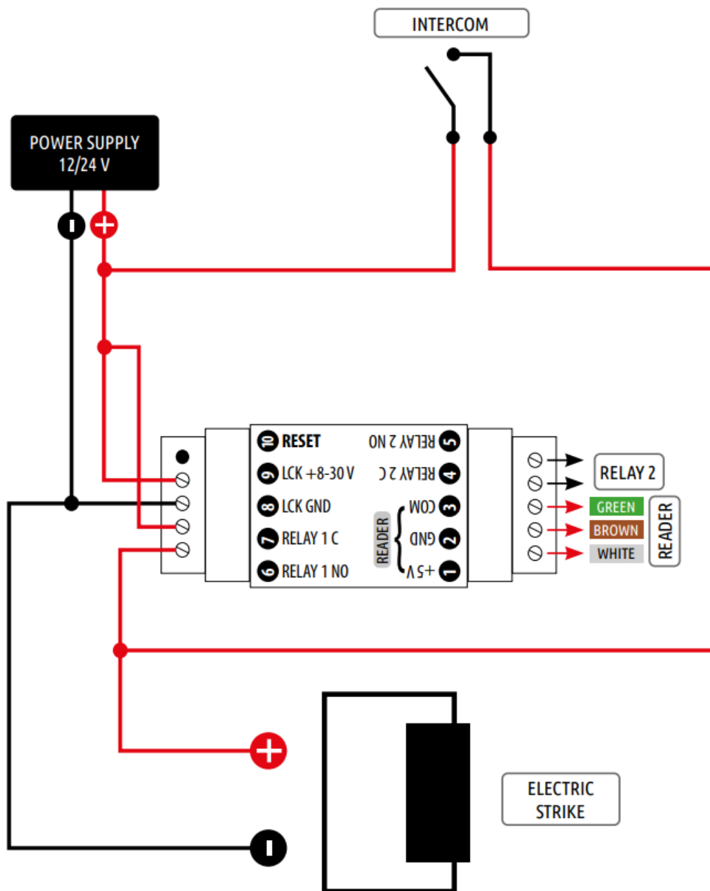
CONNECTION DIAGRAM: PRODUCTS – DIN CONTROL UNIT AND A MOTOR LOCK (ROTO ENEO)
