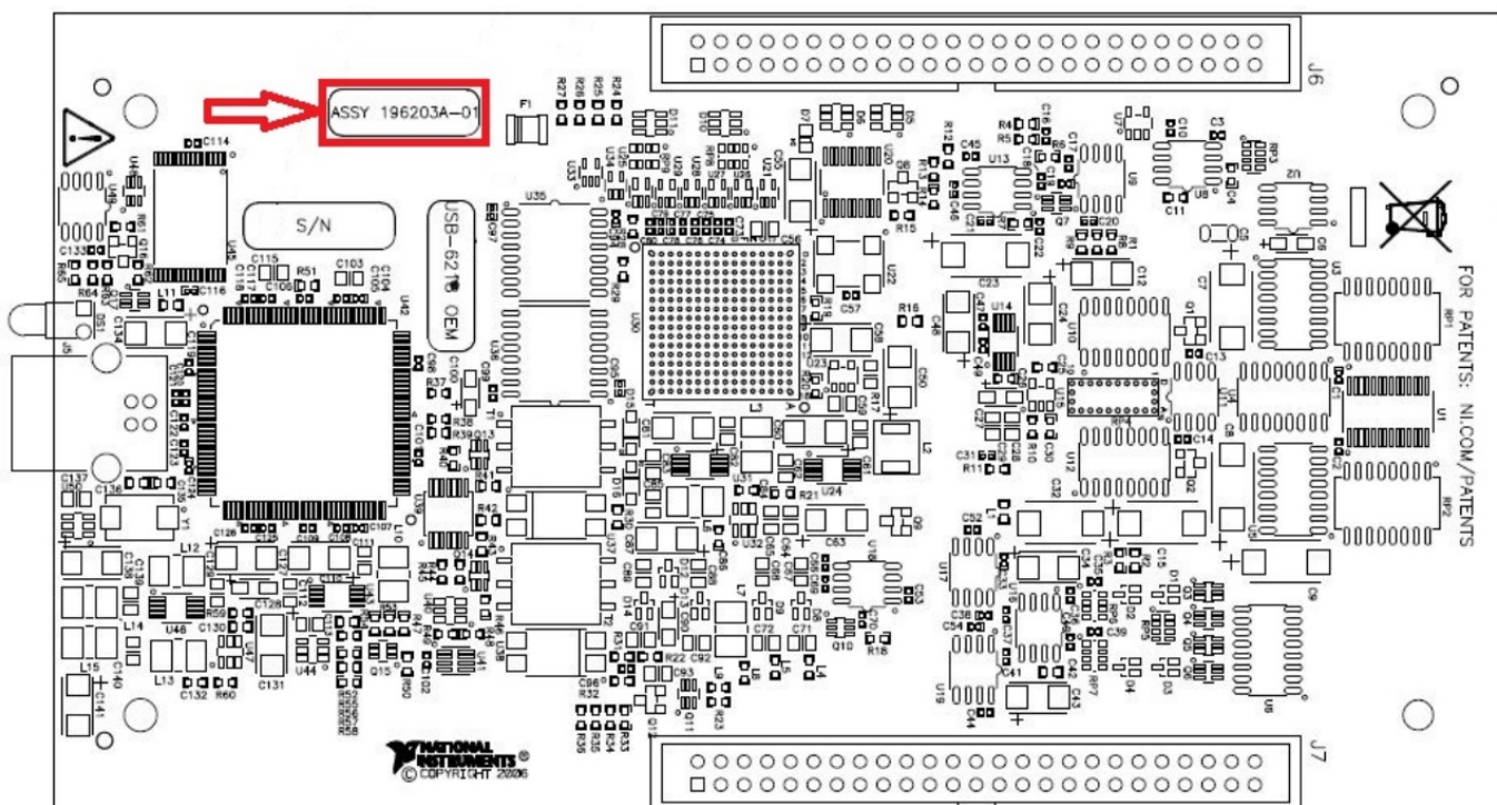
USB-6212 OEM/6216 OEM – Secondary Side
