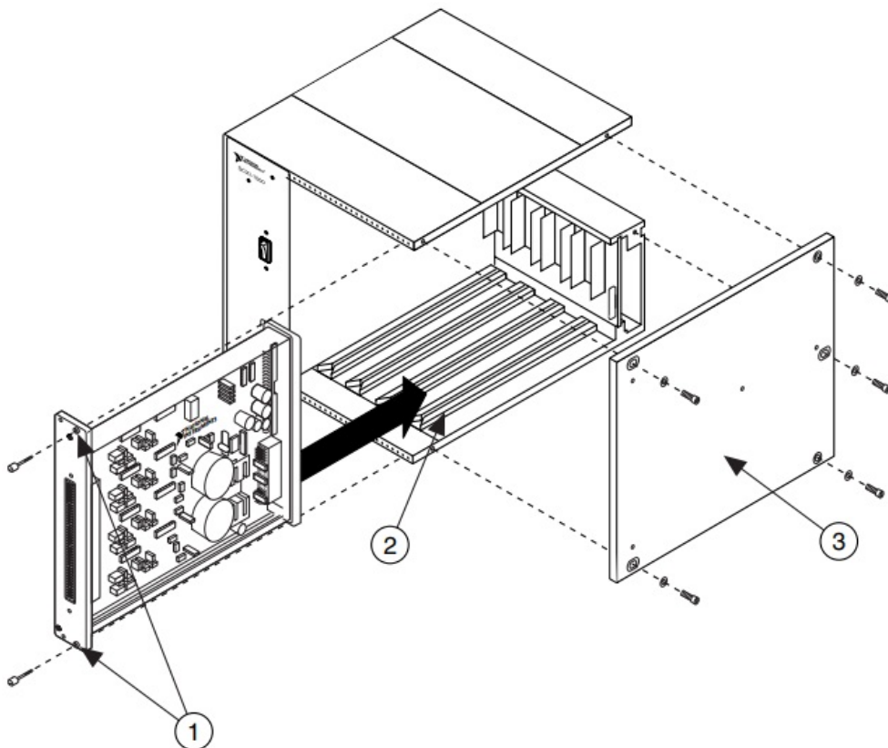
Figure 2. Side Plate Removal and Module Installation
