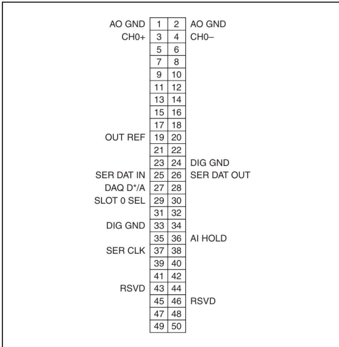
Figure 2. SCXI-1100 Rear Connector Pin Assignments
