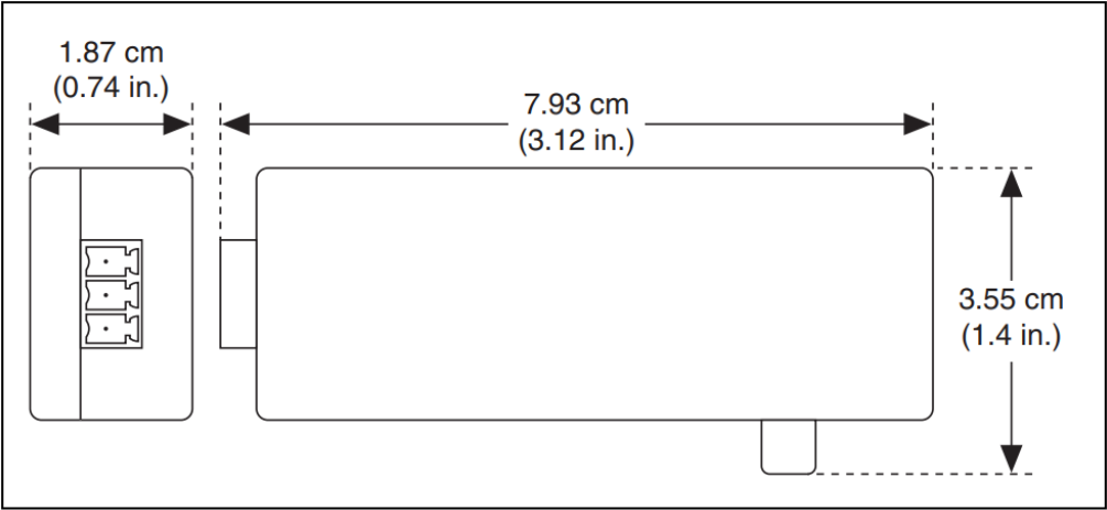
Figure 3. SCC-RLY01 Dimensions
