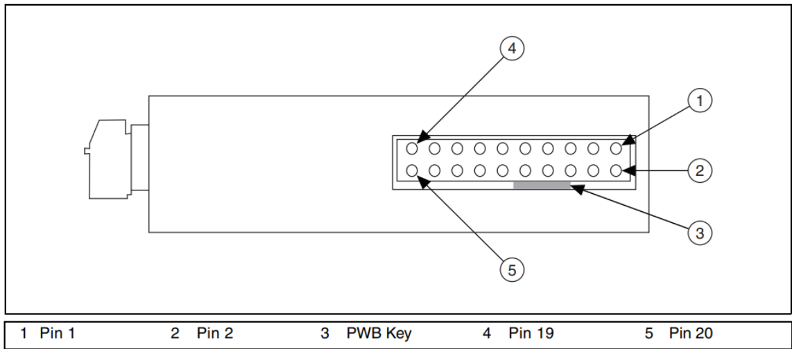
Figure 4. SCC Module Bottom View
