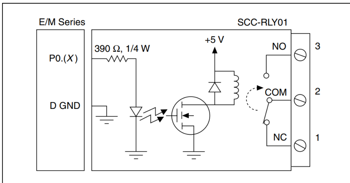
Figure 1. SCC-RLY01 Circuit Diagram
