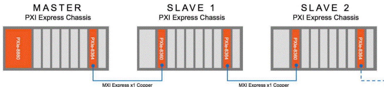
Figure 4. A PXIe-8364 host interface module is placed in a peripheral slot of the master chassis containing an embedded controller. An additional chassis is daisy chained by connecting the PXIe-8364 to a PXIe-8360 in the system controller slot of the slave chassis. Additional modules may be used to daisy-chain up to eight chassis.
