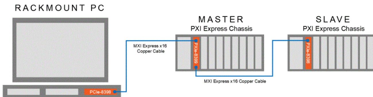
Figure 6. An NI rackmount controller is connected to a master chassis using PCIe-8398 and PXIe-8399. The PXIe-8399 features additional ports and modular cabling for daisy-chaining. An additional chassis is added to the system by connecting the PXIe-8399 to a PXIe-8398 in the slave chassis. Note that if an additional chassis were required, the PXIe-8398 could be replaced with another PXIe-8399, allowing for further expansion.
