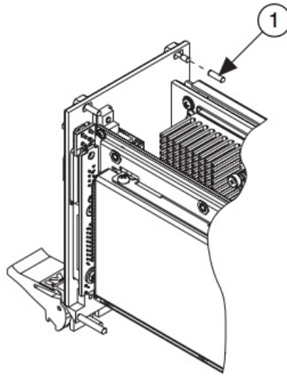
Figure 1. Removing Protective Screw Caps
