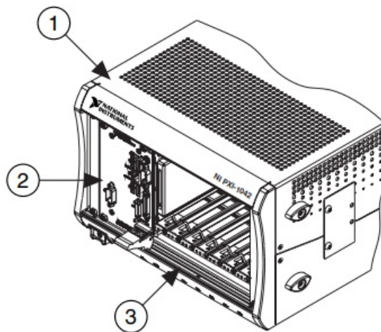
Figure 2. NI 8195/8196 Installed in a PXI Chassis
