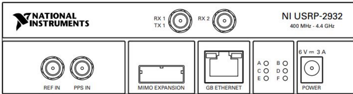
Figure 3. NI USRP-2932 Front Panel
