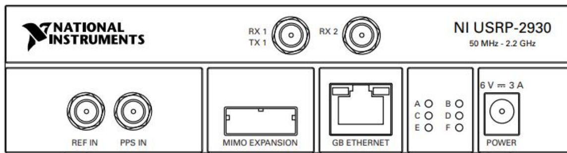
Figure 1. NI USRP-2930 Front Panel
