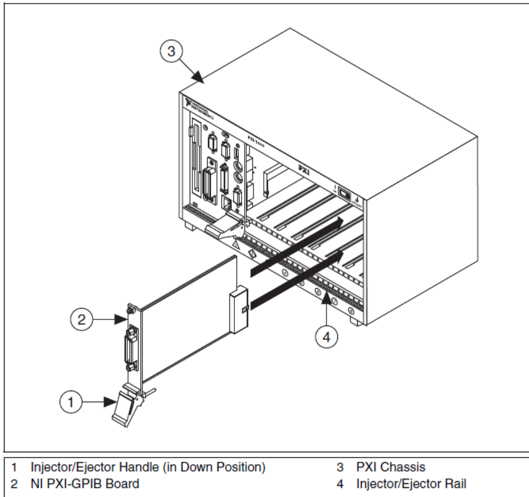
Figure 2. Installing the NI PXI-GPIB
