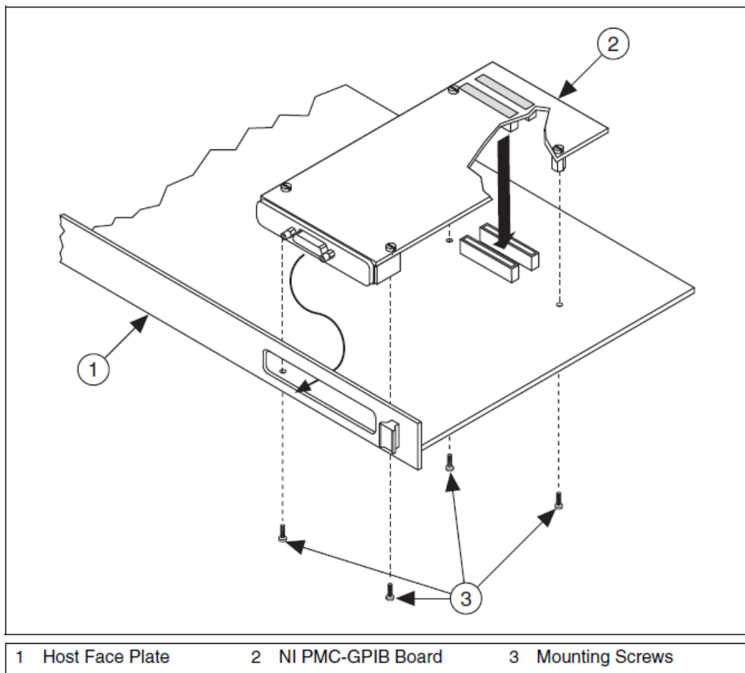
Figure 3. Installing the NI PMC-GPIB
