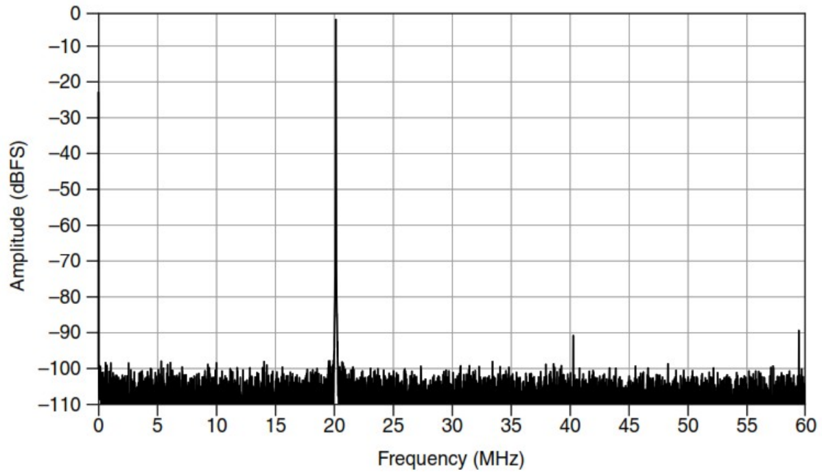
Figure 4. Analog Input One-Tone Spectral Measurement (20.17 MHz, -1 dBFS)
