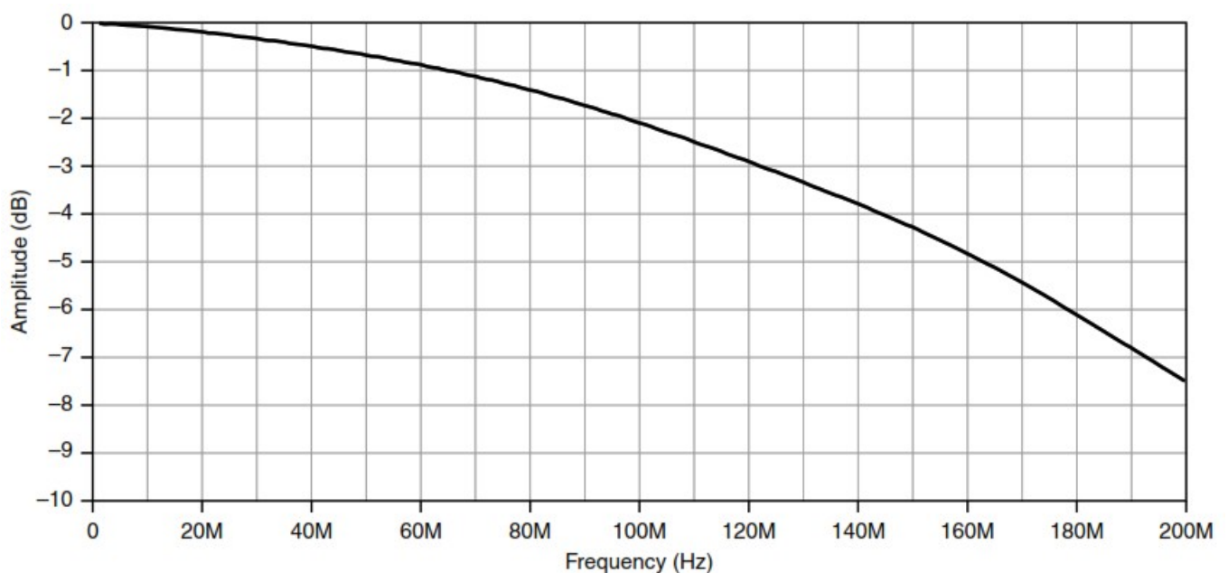
Figure 3. DC-Coupled Passband
