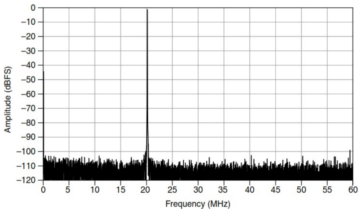
Figure 2. Analog Input One-Tone Spectral Measurement (20.17 MHz, -1 dBFS)
