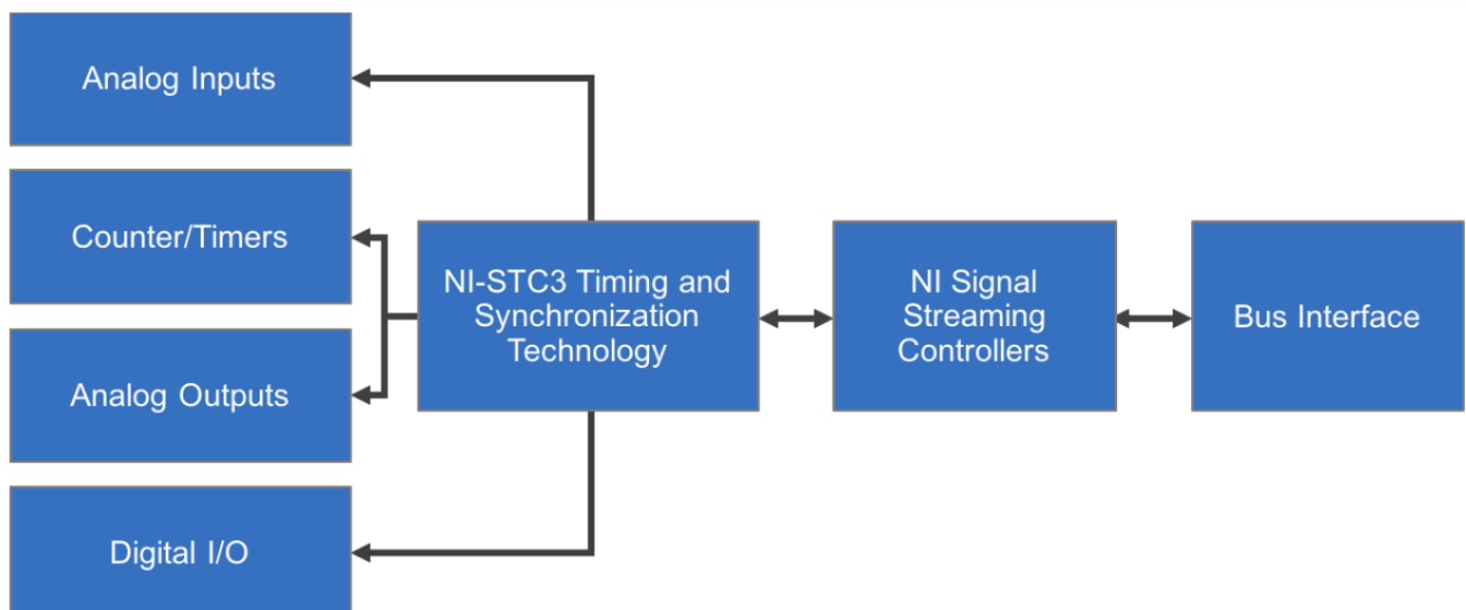
Figure 1. Modern NI DAQ devices feature NI-STC3 timing and synchronization technology – a USB Multifunction I/O Device is shown here as an example.
