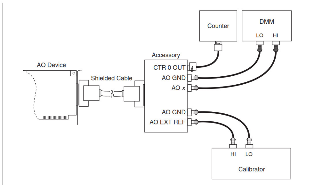
Figure 1. Calibration Connections
