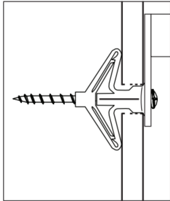
4. Tighten to 100%
