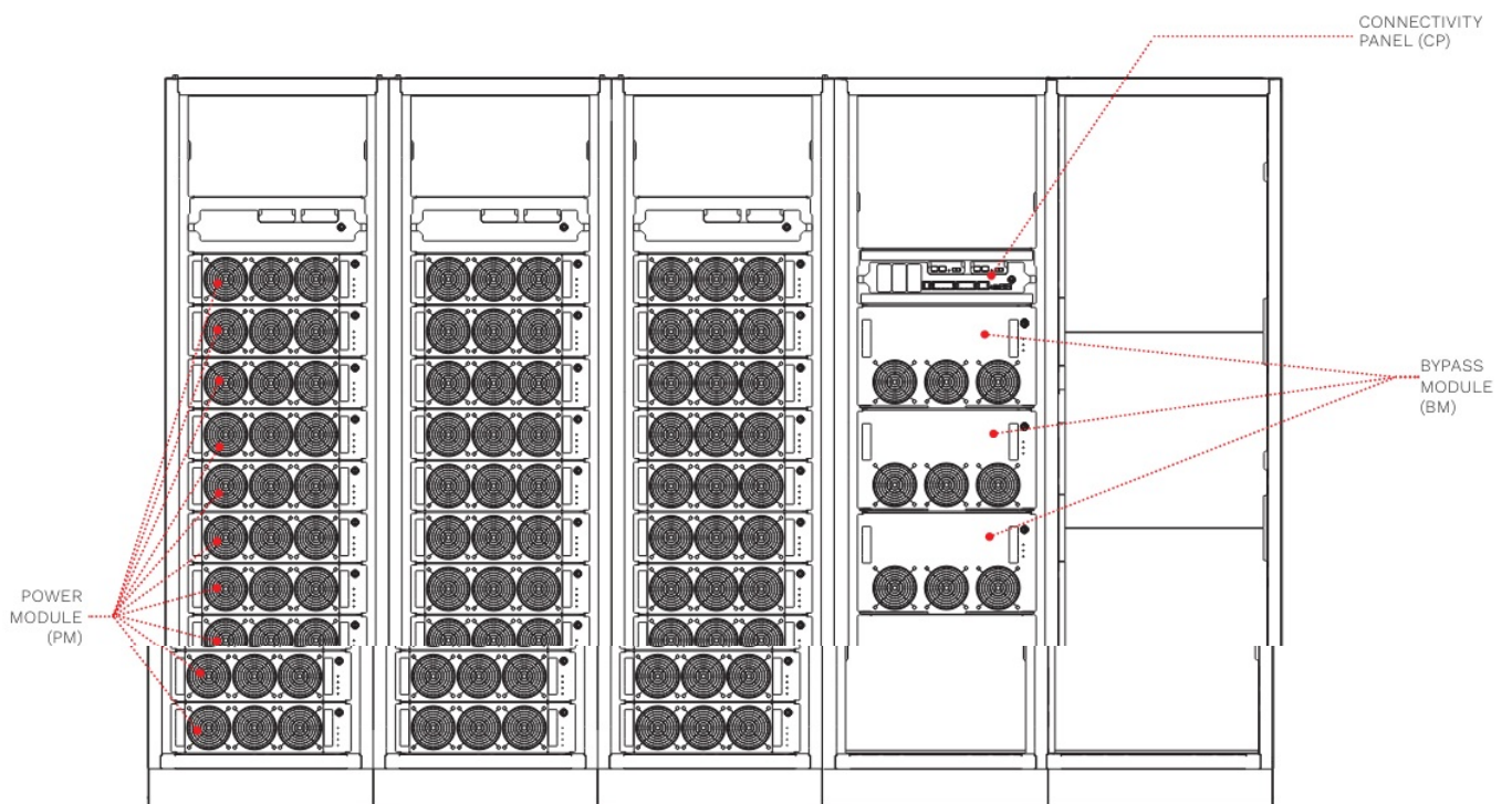
M2S 1600 PCS with input, bypass, output and manual bypass switches up to 1600 kW (front)
