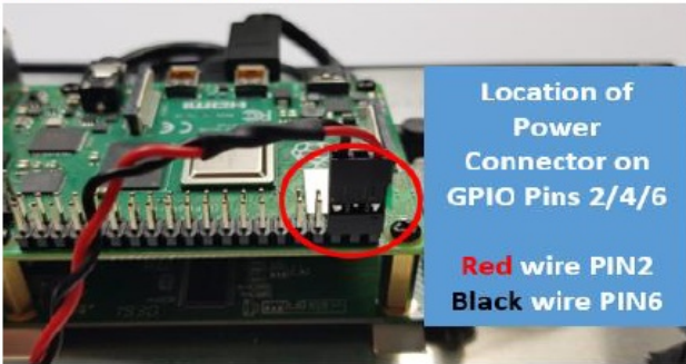
Item#5 – Internal Power Connector
