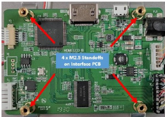
Standoffs x 4 location on interface PCB (#1)
