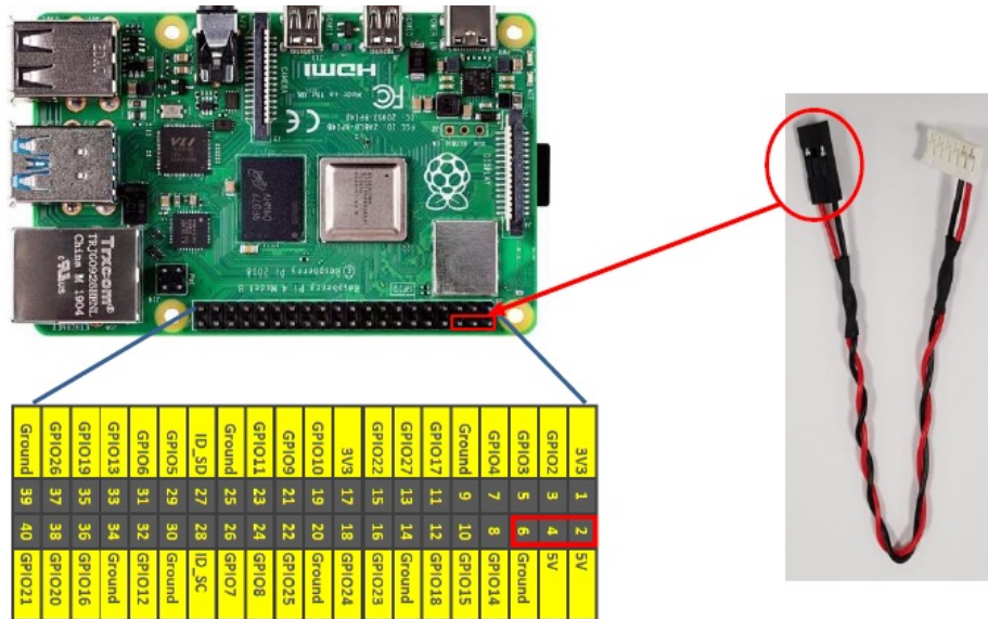
Item#5 – Internal Power Connector
