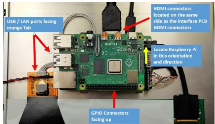
Top View position with PI4 mounted (#2)
