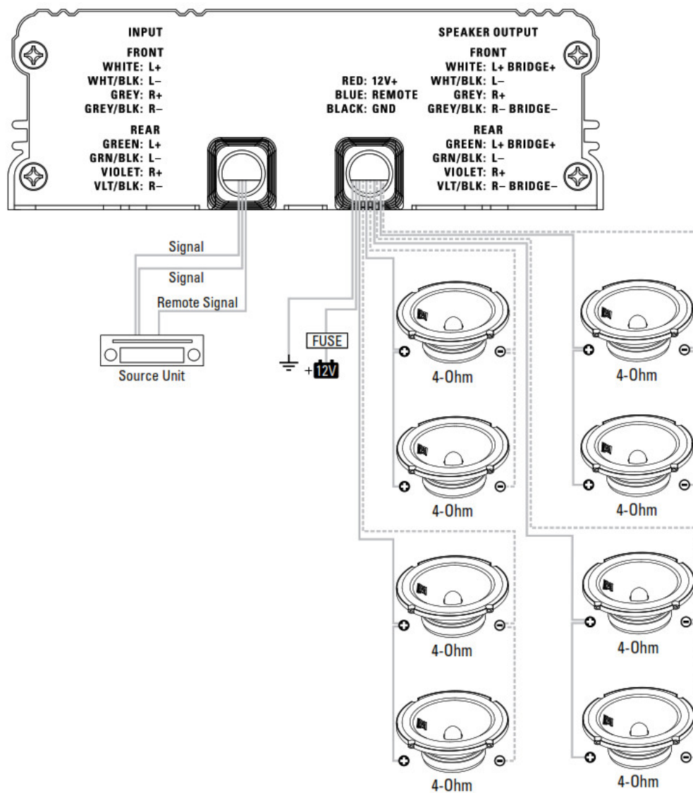
WIRING DIAGRAM Stereo 4 \Omega Front/4 \Omega Bridged Rear
