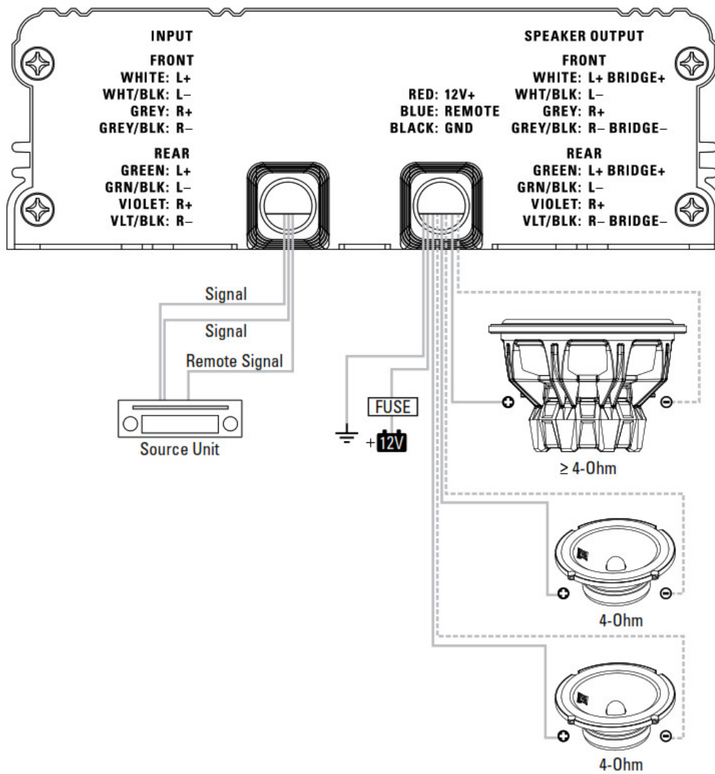
WIRING DIAGRAM 4Ω Bridged Subwoofers
