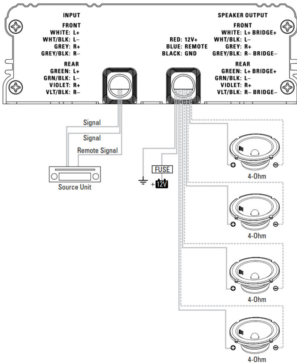
WIRING DIAGRAM 2Ω Stereo
