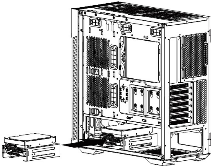
2.5" SSD , HDD Installation/ 2.5" SSD
