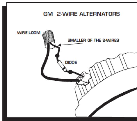
Figure 7 Installing the Diode to a 1973-1983 GM Vehicle.
