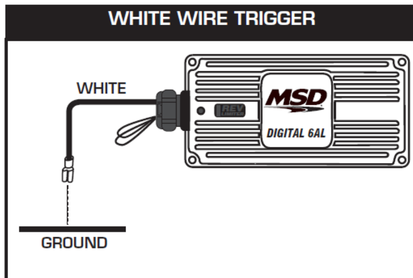
Figure 9 Checking for Spark with the White Wire.
