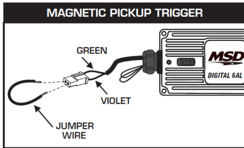
Figure 10 Checking for Spark with the Mag Pickup.
