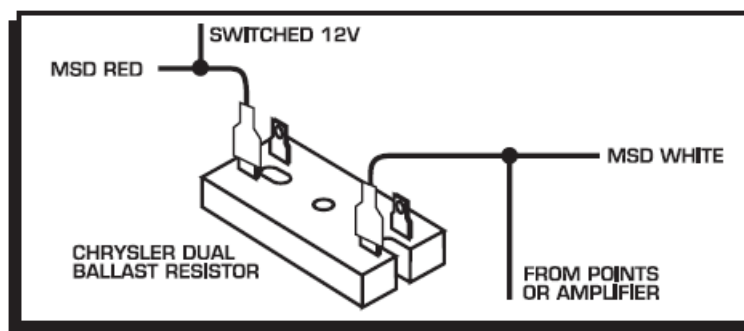
Figure 5 Wiring the Dual Ballast Resistor.
