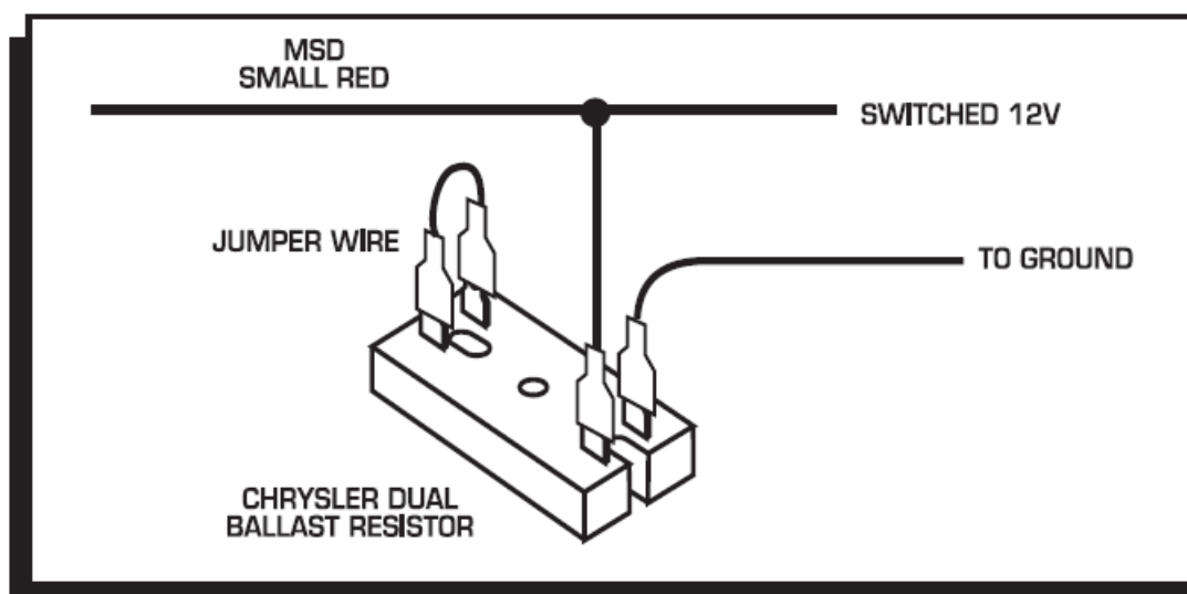
Figure 8 Wiring the Dual Ballast Resistor for Run-On.
