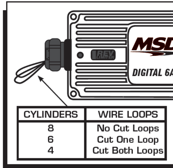
Figure 1 Programming the Number of Cylinders.
