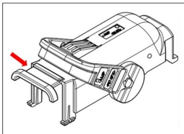
Figure 1: Cover as in the connector kit. The red arrow marks the groove in which the cable harness sheath must
