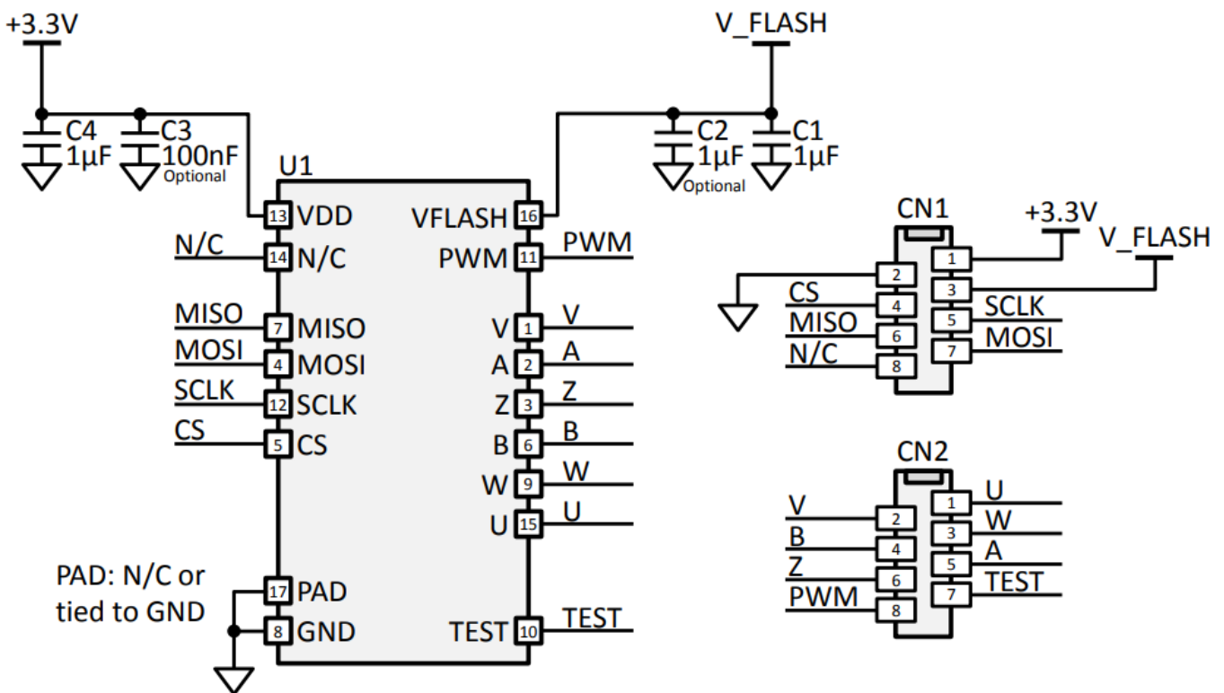
Figure 5: Schematic Type 1
