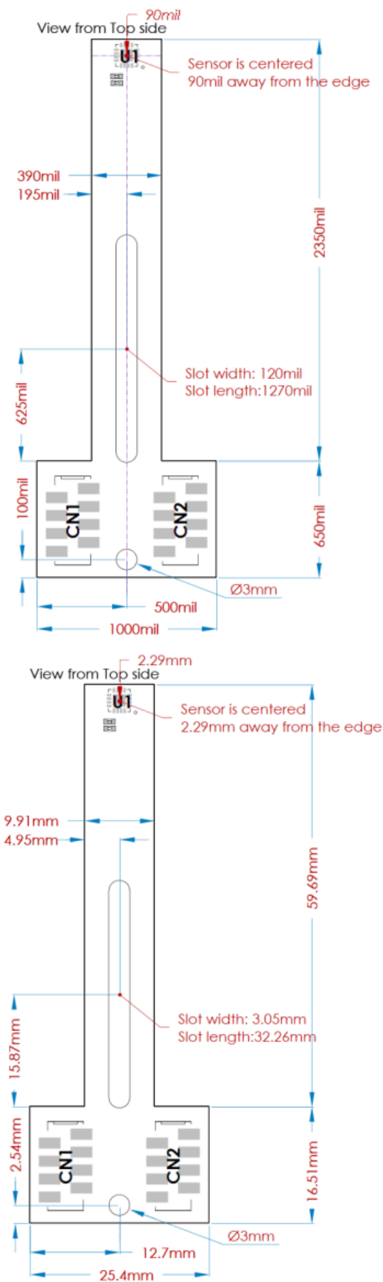
Figure 18: Mechanical Drawing LT Type 2 mil = 0.001in = 0.0254mm
