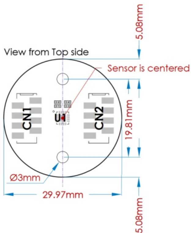
Figure 8: Mechanical Drawing RD Type 1
