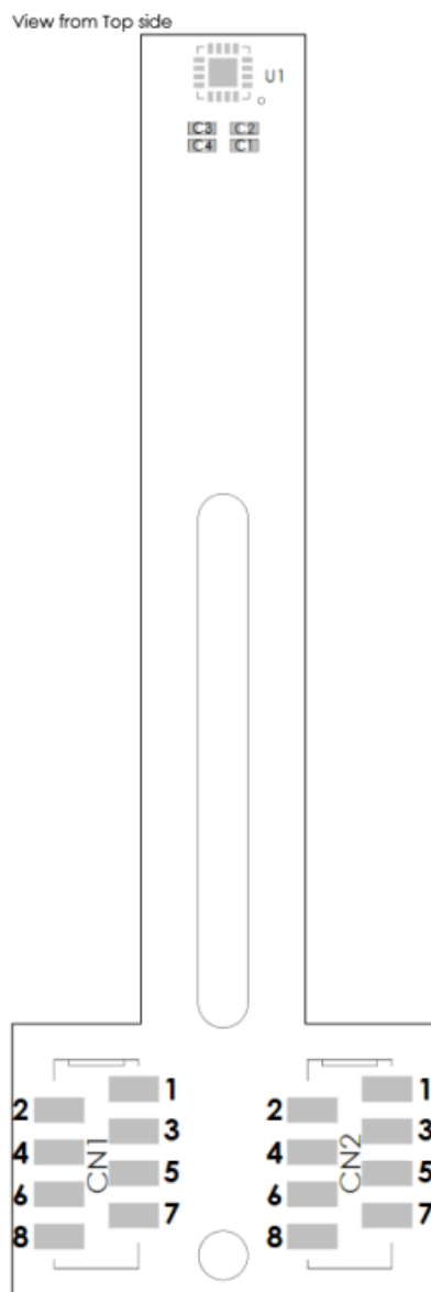
Figure 11: Connector LT Pinout Type 1
