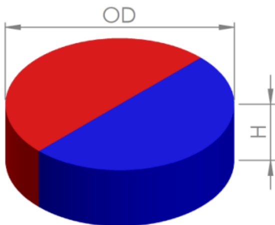
Figure 21: Cylinder Magnet, Diametrically Magnetized
