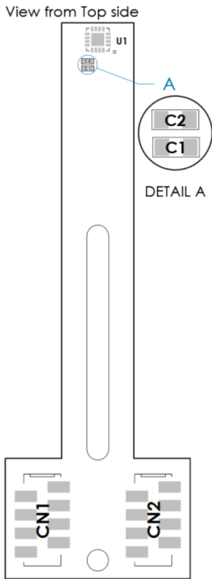
Figure 16: Assembly View LT Type 2
