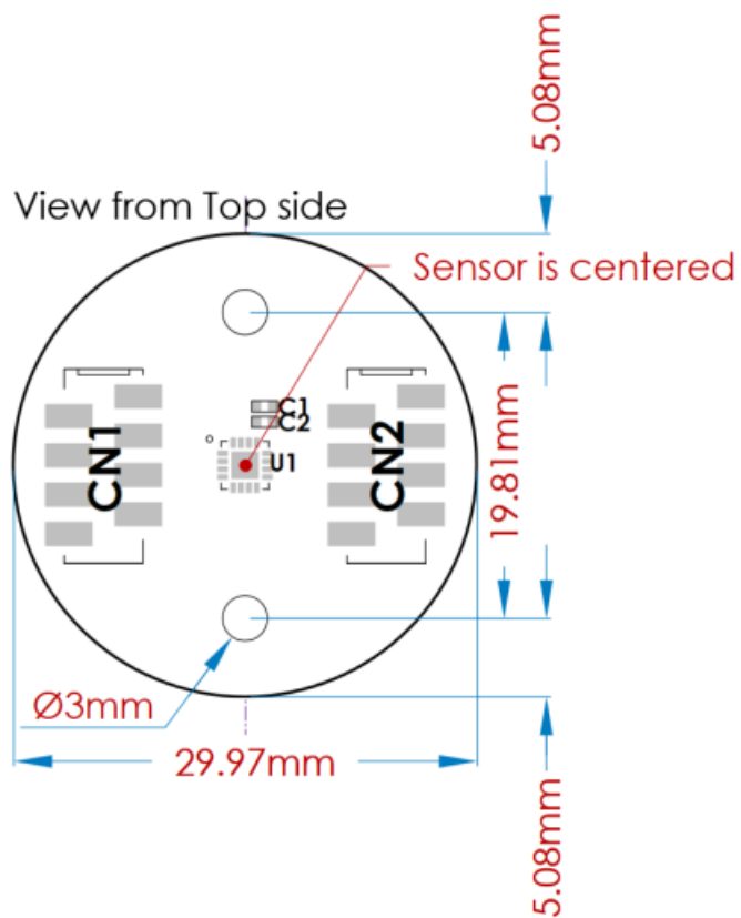
Figure 17: Mechanical Drawing RD Type 2
