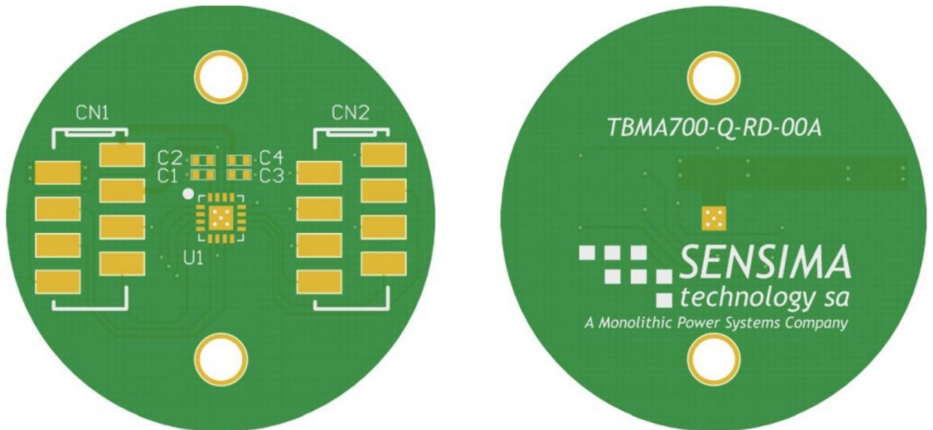
Figure 3: RD Board Overview Type 1
