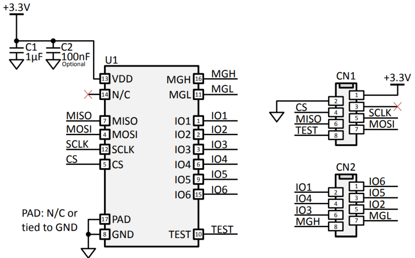
Figure 14: Schematic RD/LT Type 2
