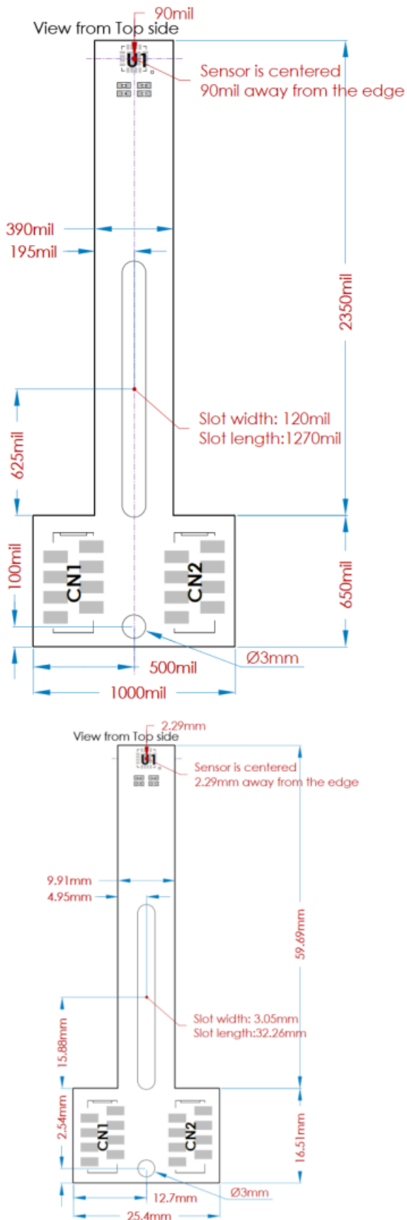
Figure 9: Mechanical Drawing LT Type 1 mil = 0.001in = 0.0254mm
