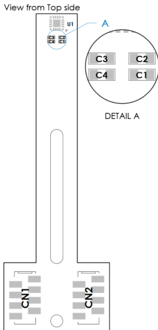
Figure 7: Assembly View LT Type 1
