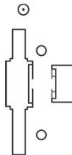
SD card slot without upper case
