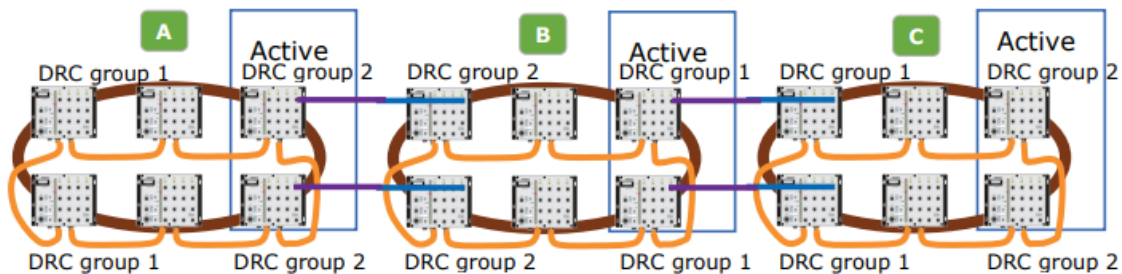
Turbo Ring V2 with DRC Diagram 1
