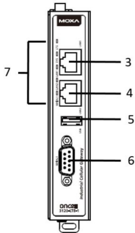
Bottom Panel View
