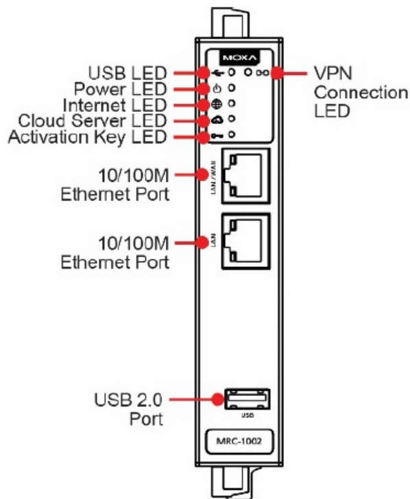
MRC-1002
