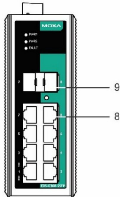
EDS-G308-2SFP Front Panel View
