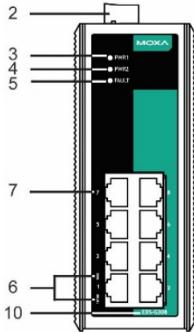
EDS-G308 Front Panel View
