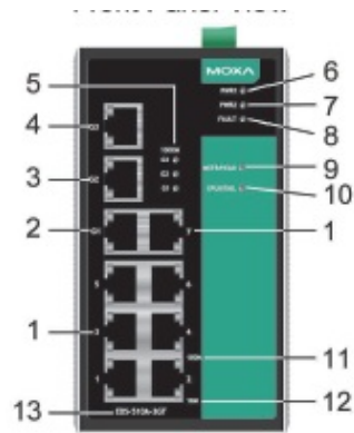
EDS-510A-1GT2SFP Front Panel View
