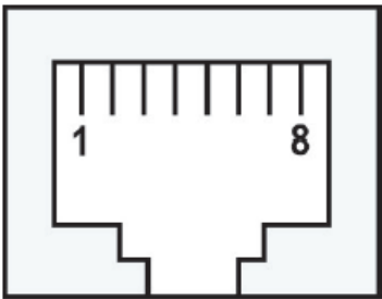
RJ45 (8-pin) to RJ45 (8-pin) Straight-Through Cable Wiring
