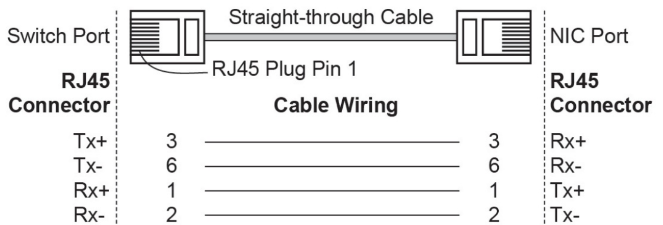
RJ45 (8-pin) to RJ45 (8-pin) Cross-Over Cable Wiring
